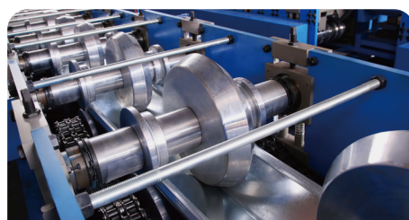
Forming rollers
