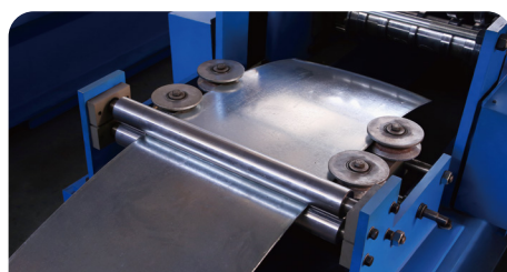
Feed guide
