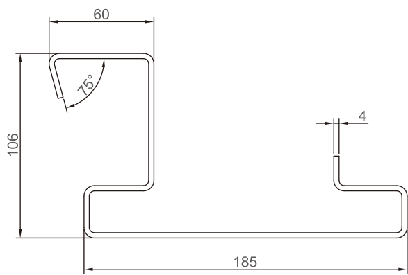
Hydraulic post-punching
